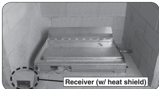
Fig. 14-4 Place remote receiver
