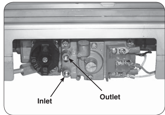
Fig. 18-1 12 valve: check pressure
