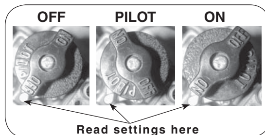
Fig. 15-1 12 valve operating positions
