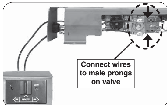
Fig. 14-3 Connect remote receiver to valve
