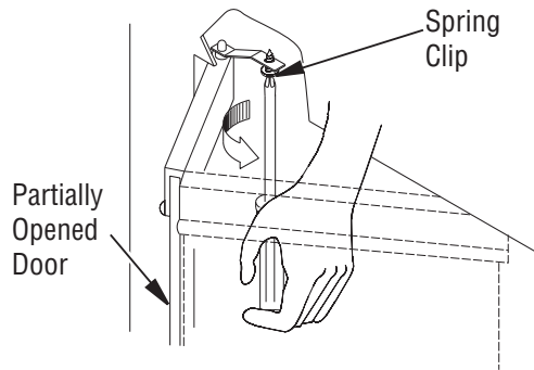
Figure 9: Door Adjustment
