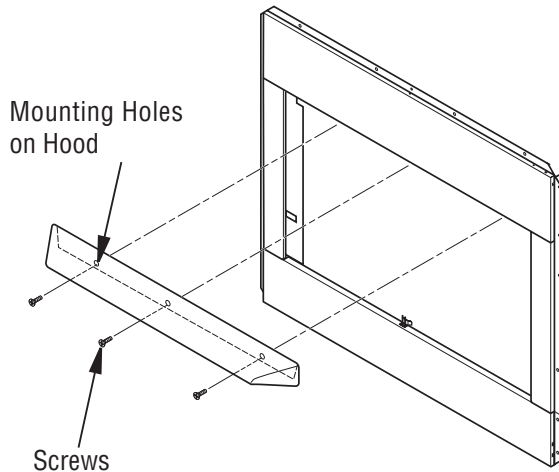
Figure 7 - Installing Hood
