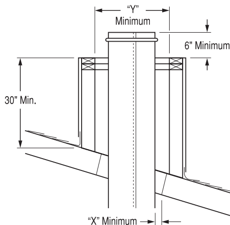
Figure 3 - Constructing Chase (RT(L)-8 Series Only)
