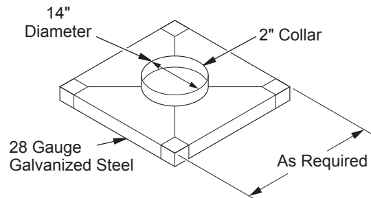
Figure 4 - Constructing Chase Top Flashing
