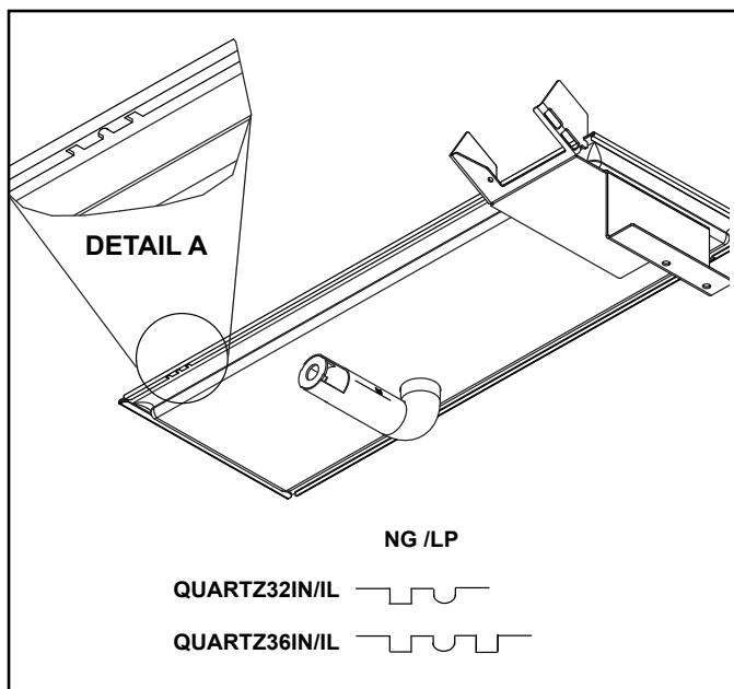
Figure 9.2 Burner Identification
