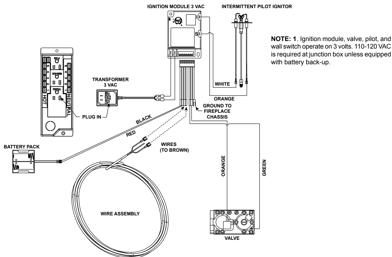
Figure 8.2 Intellifire Pilot Ignition (IPI) Wiring Diagram with Wall Switch or Thermostat (Standard)
