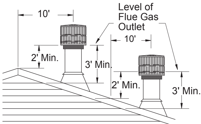
Figure 25 - 10 Foot Rule
