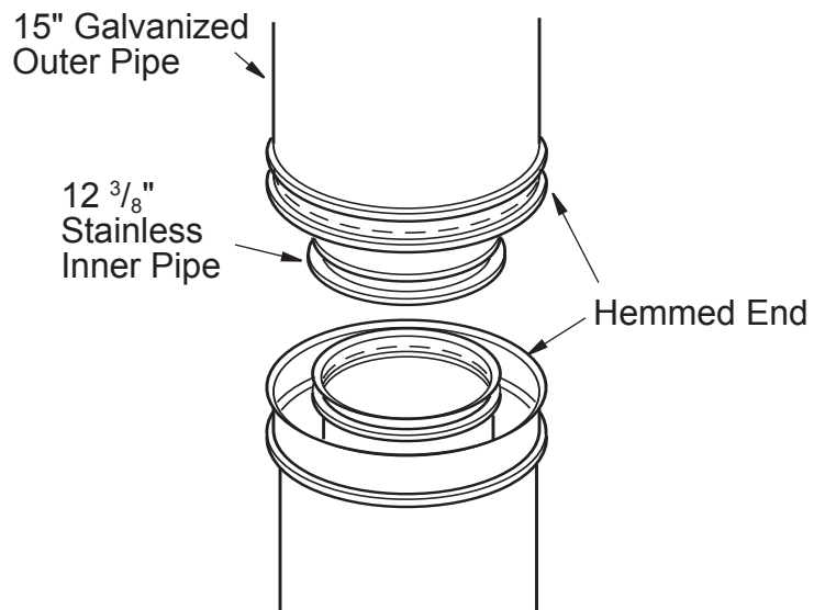
Figure 14 - Lineal Gain
