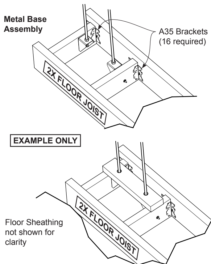
Figure 26 - Floor Joist Installation
