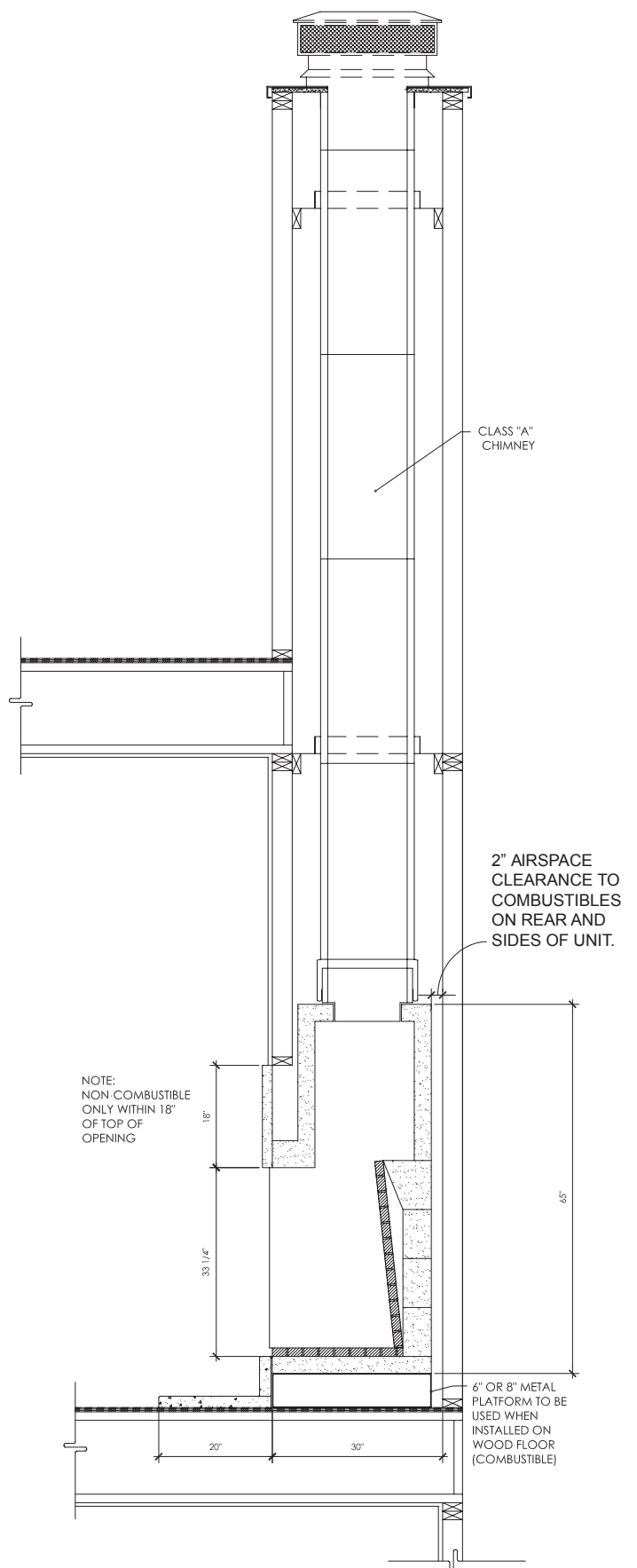
Figure 12: Combustible Floor
