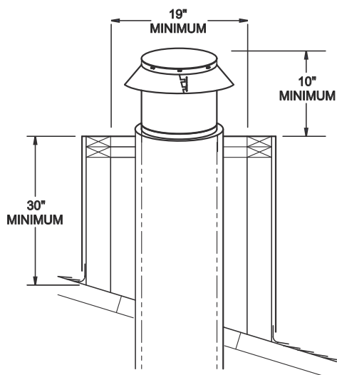
Figure 1 - Constructing Chase
