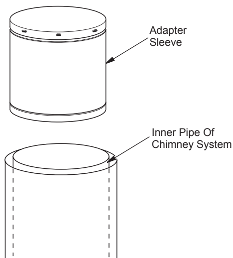
Figure 2 - Installing Adapter Sleeve
