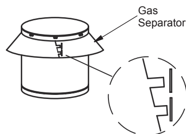
Figure 3 - Installing Gas Separator
